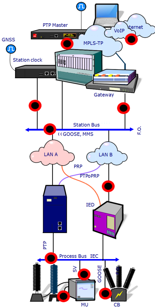
Fig2. Testing points.
